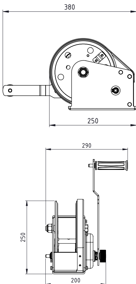
40401/40408 - Hand Winch with mounting bracket kit
