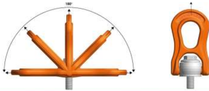
Permitted directions of pull
