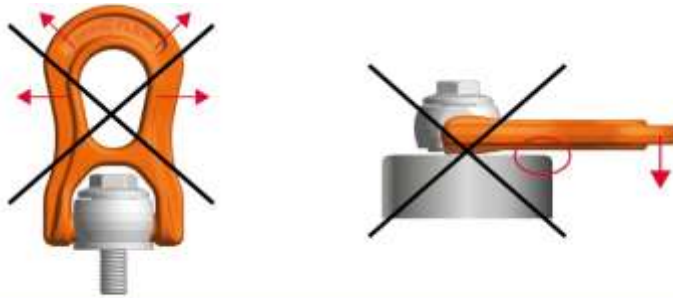
Non-permitted directions of pull
